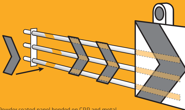
Powder coated panel bonded on GRP and metal posts with Sikaflex®-552 AT . For faster curing, Sikaflex®-953 can be used. For UV-resistant or primer-free applications, Sikasil® AS-70 or the fast cure Sikasil® AS-785 are advised.
