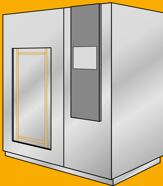
Bonding of a stainless steel door to the frame: Sikaflex®-552 AT . For faster assemblies, Sikaflex®-953 can be used.
