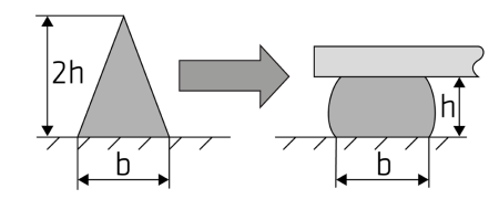
Figure 1: cordon triangulaire recommandé
