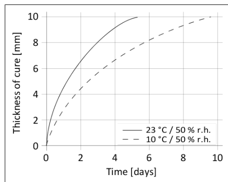
Diagram 1: curing speed Sikaflex®-298
